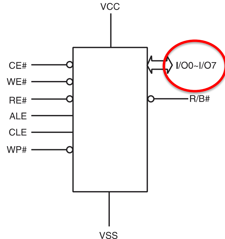
NAND Flash
