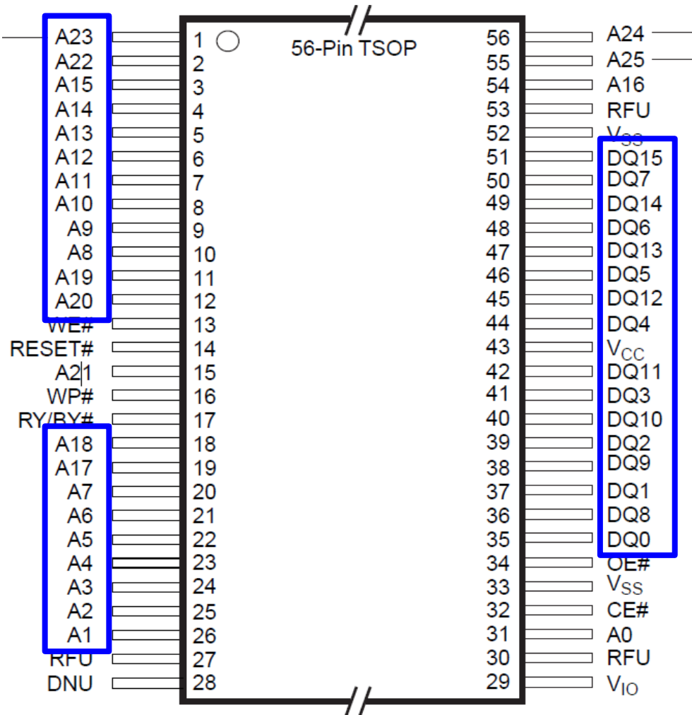
NOR Flash
